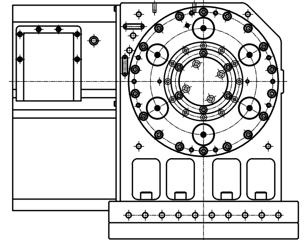
[ MTR2-25440YY Specifications ]
